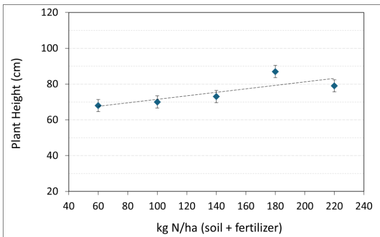
Figure 12. Nitrogen rate effects on quinoa plant height at Swift Current, 2024. The primary N source was side-banded urea. The overall F-test ( P = 0.017 ) and linear orthogonal contrast ( P = 0.002 ) results were significant.
