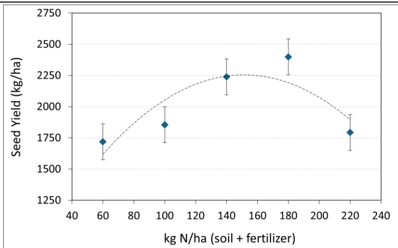
Figure 10. Nitrogen rate effects on quinoa grain yield at Outlook, 2024. The primary N source was side-banded urea. The overall F-test ( P = 0.031 ) and quadratic orthogonal contrast ( P = 0.005 ) results were significant.
